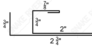
"F" Channel ( \frac{3}{4} " x \frac{3}{4} " )
