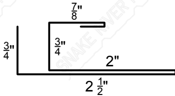
"F" Channel ( \frac{1}{2} " x \frac{3}{4} " )
